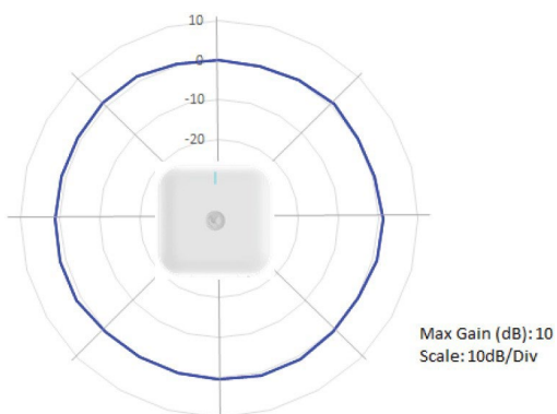
4x4 5 GHz Azimuth
